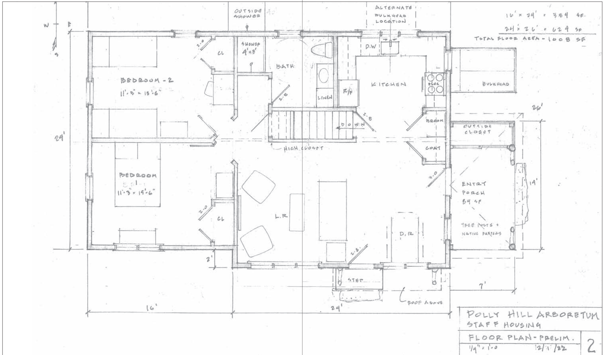
Figure 5 Single-family Floor Plan
