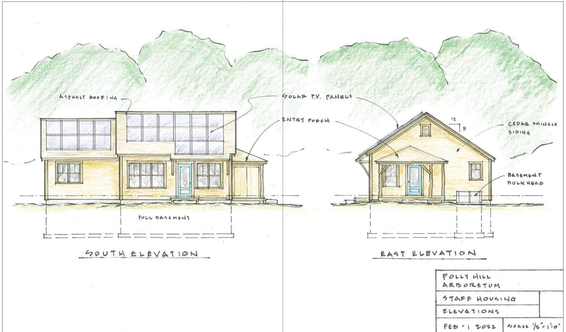
Figure 4 House Elevations
